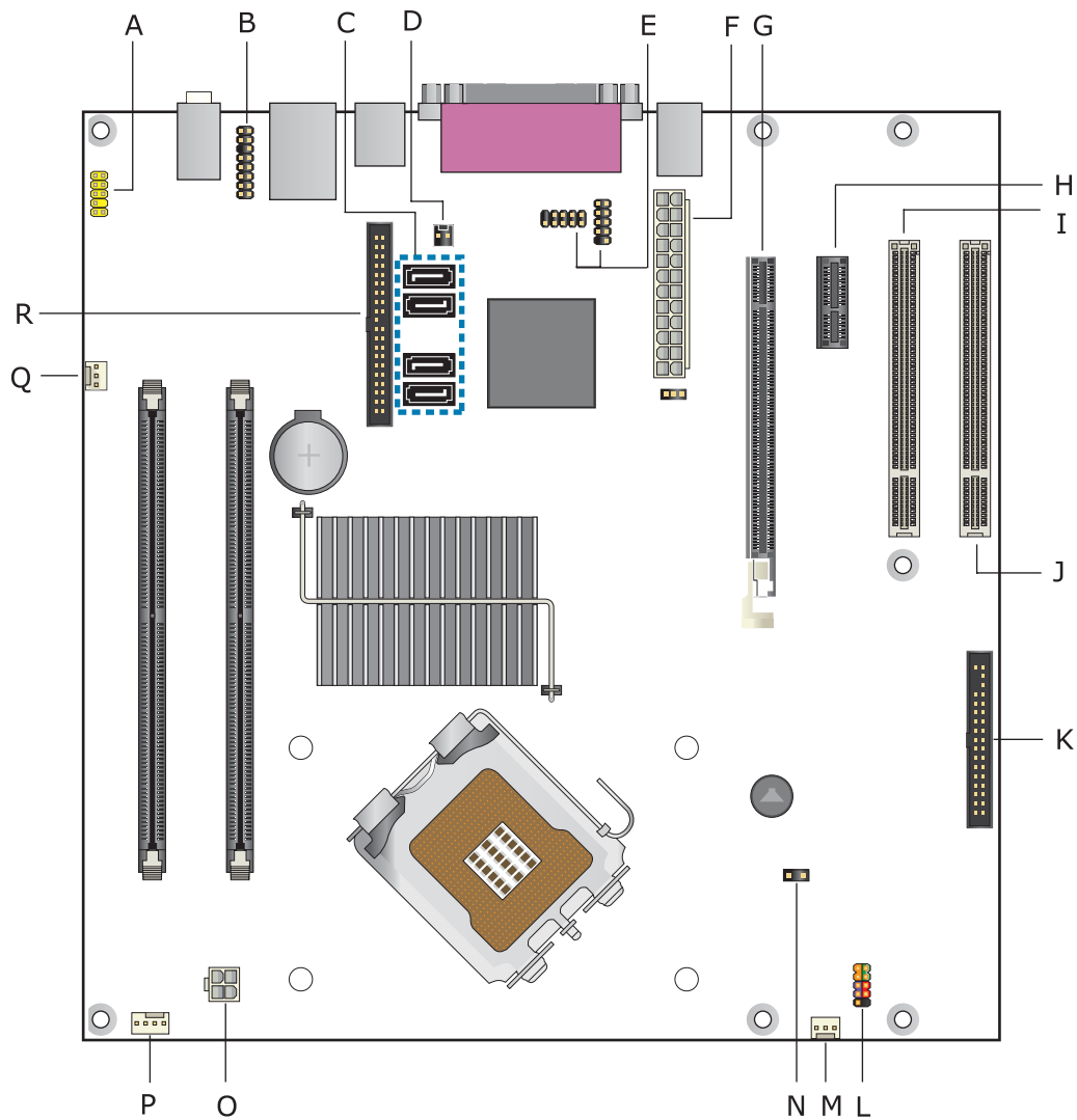
Figure 14. Component-side Connectors and Headers
