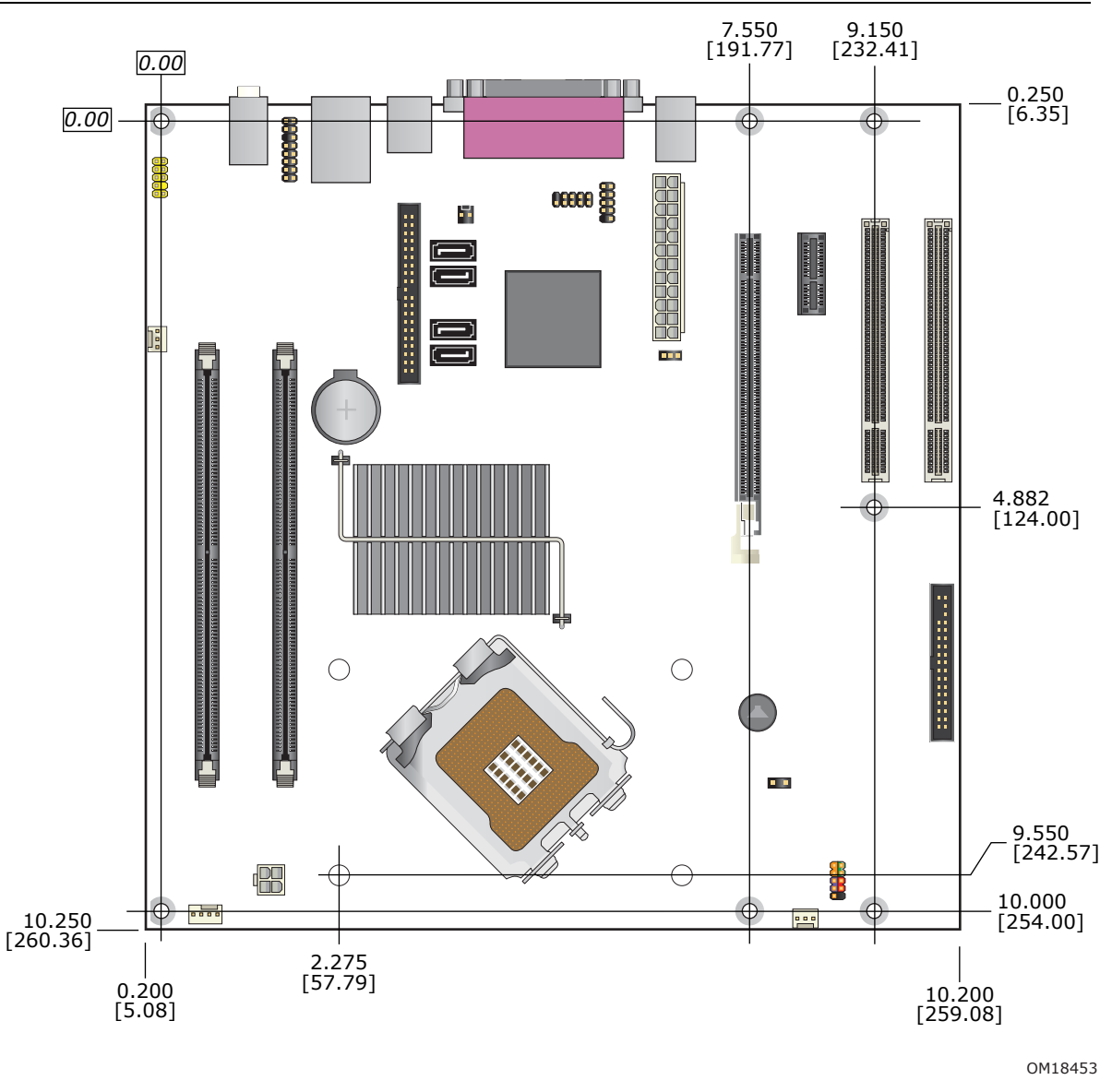
Figure 18. Board Dimensions
