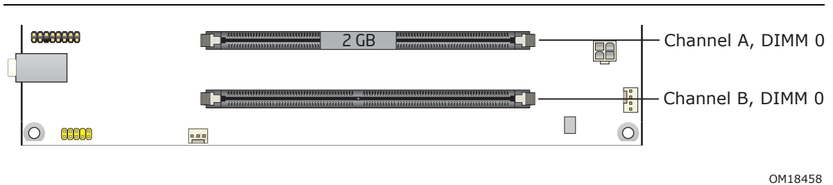
Figure 5. Single Channel (Asymmetric) Mode Configuration with One DIMM
