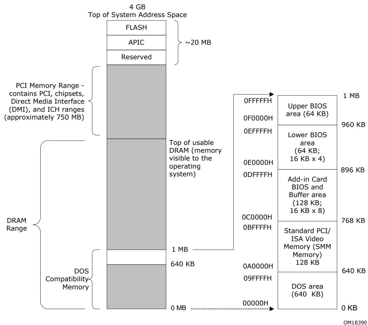
Figure 12. Detailed System Memory Address Map
