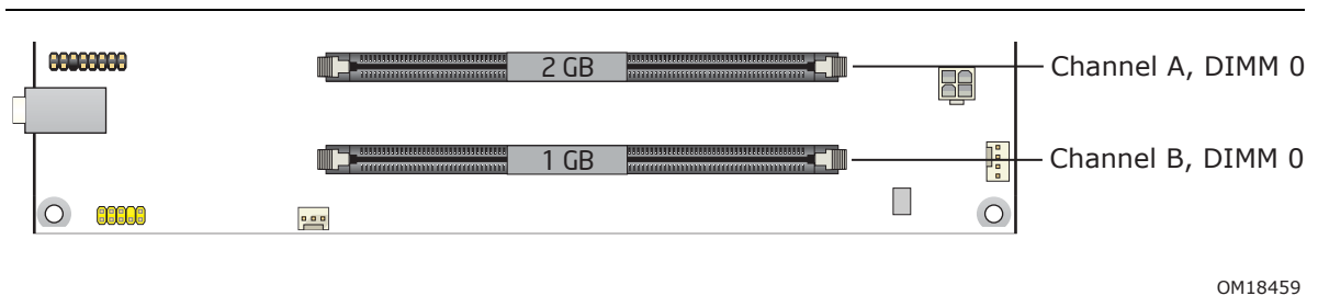
Figure 6. Single Channel (Asymmetric) Mode Configuration with Two DIMMs
