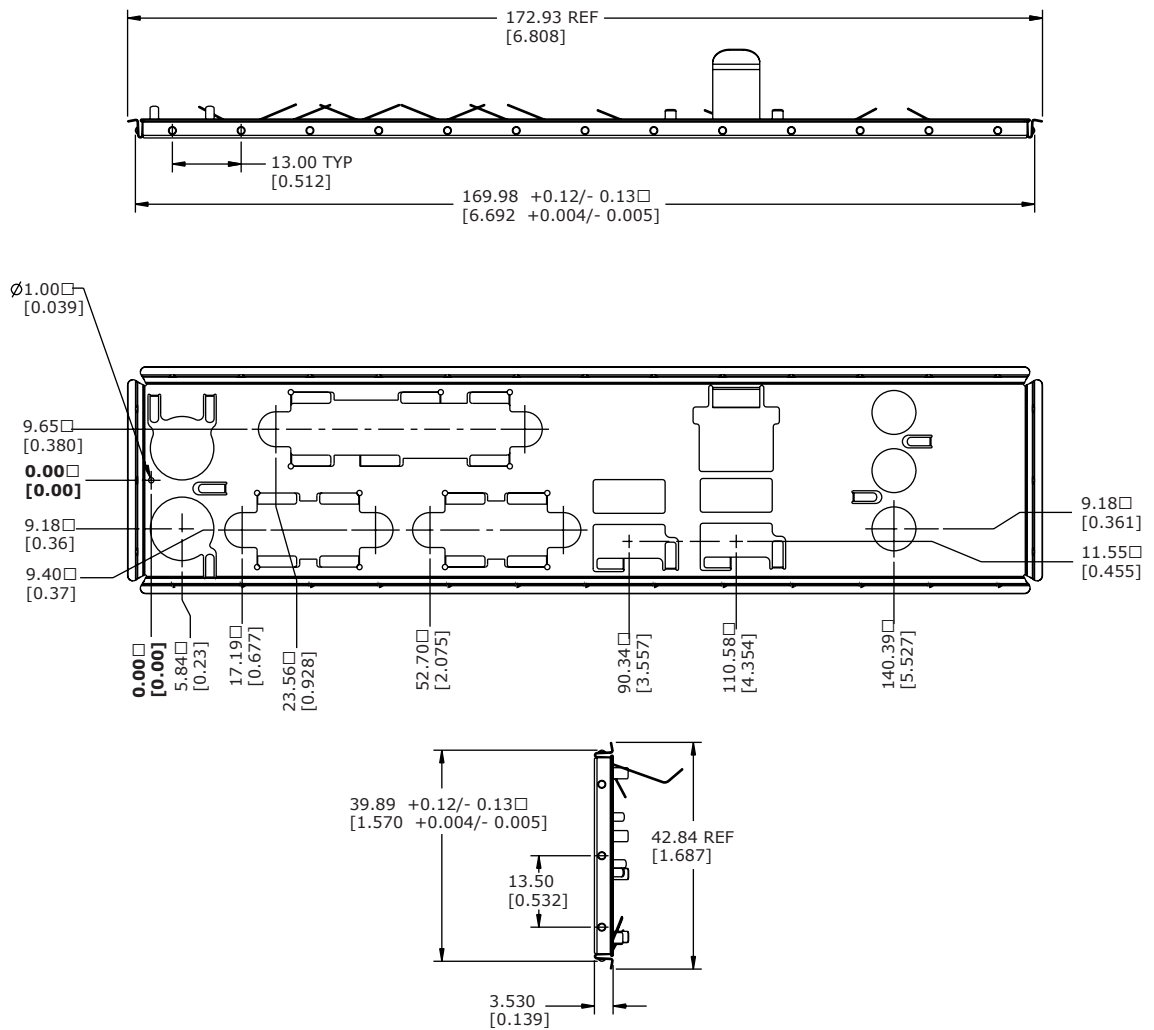
Figure 19. I/O Shield Dimensions
