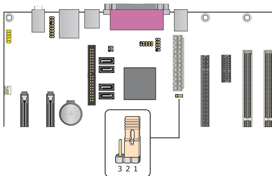
Figure 17. Location of the Jumper Block
